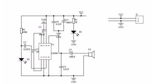
Schematic receiving end:
